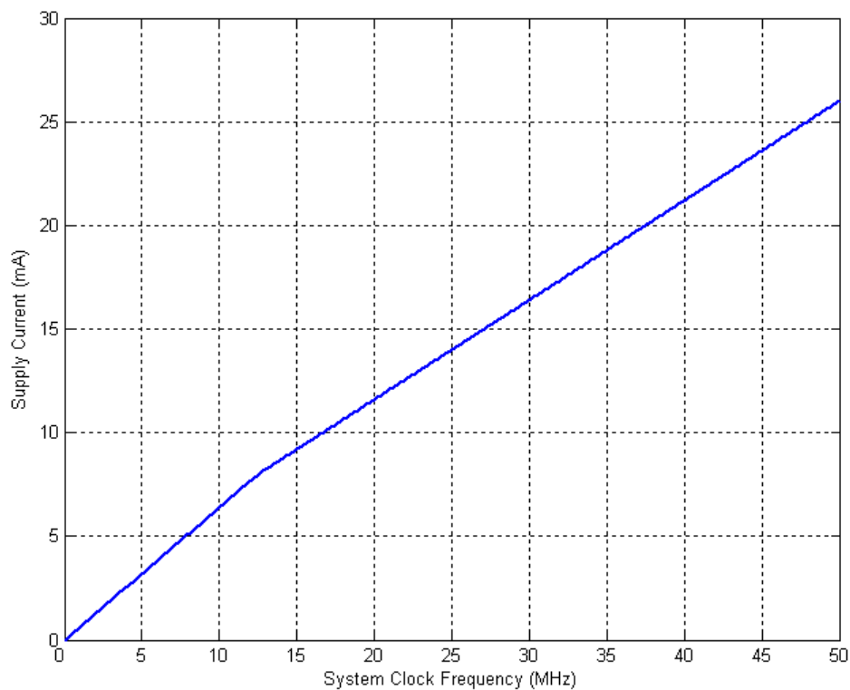
Figure 5.1. Typical Active Mode Current vs. Frequency
