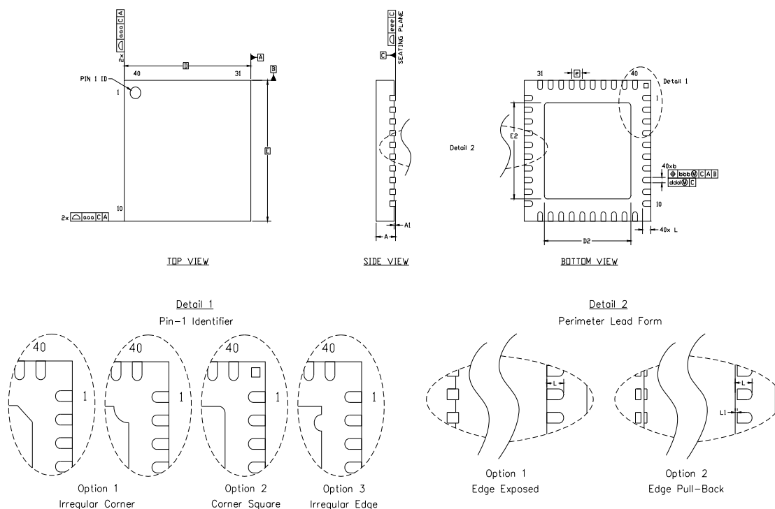
Figure 4.5. Typical QFN-40 Package Drawing
